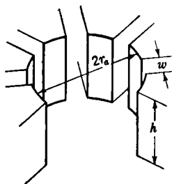
FIG. 10-3.—Anode interaction-space interface.
